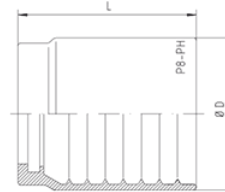
DN 31, 38, 51
